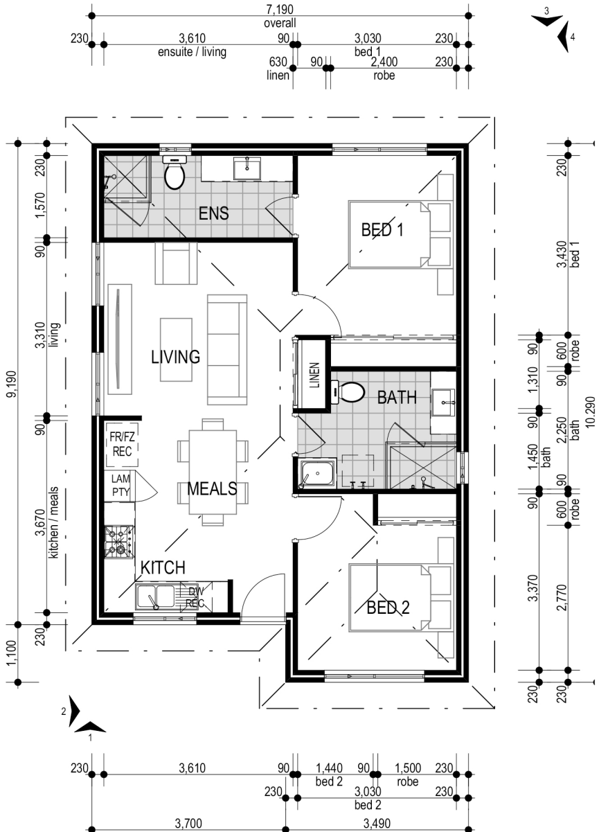
2xBED 2xBATH ANCILLARY PLAN
